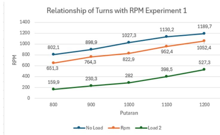
Figure 2. Relationship between Rotation and RPM Rotation Experiment 1
