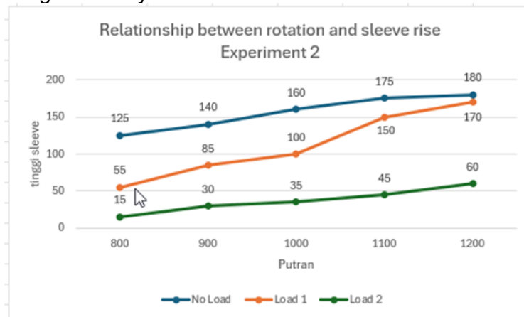
Figure 5. Relationship between Rotation and Sleeve Increase Experiment 2
