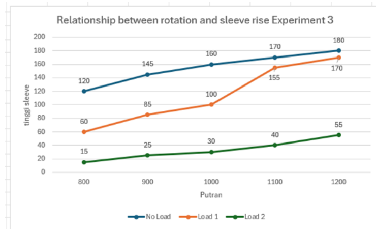
Figure 7. Relationship between Rotation and Sleeve Increase Experiment 3
