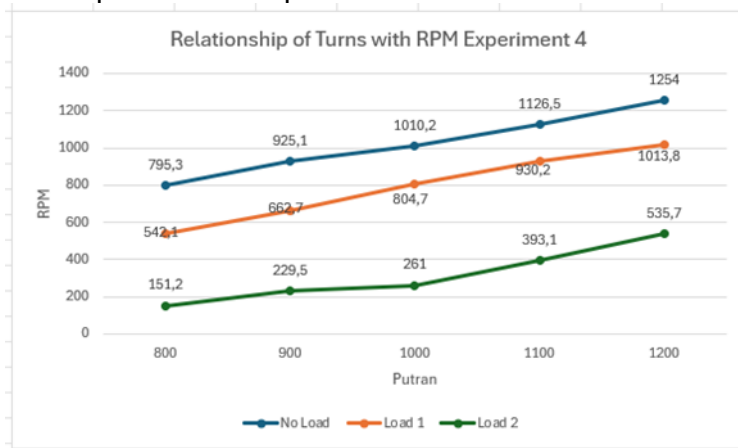
Figure 8. Relationship between Rotation and RPM Rotation Experiment 4
