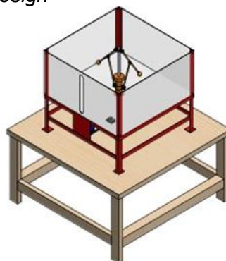
Figure 1. Governor test equipment design
