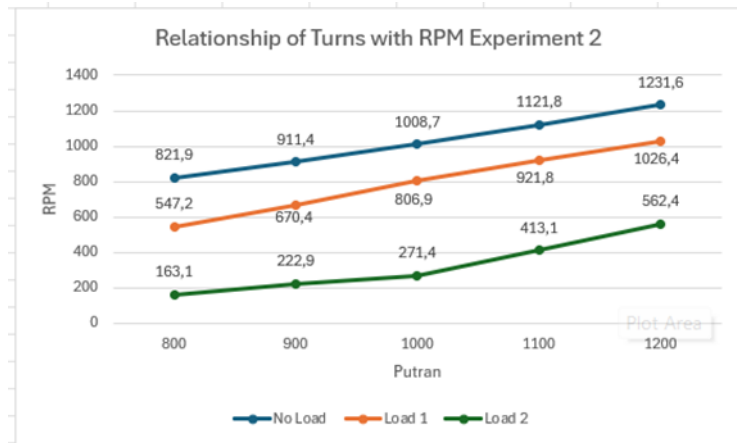
Figure 4. Relationship between Rotation and RPM Rotation Experiment 2
