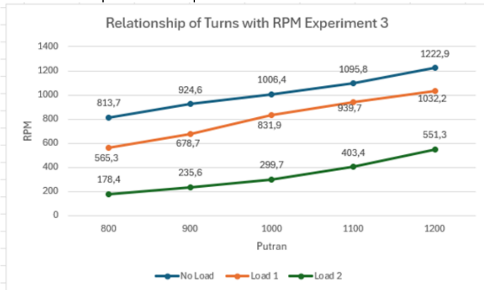
Figure 6. Relationship between Rotation and RPM Rotation Experiment 3
